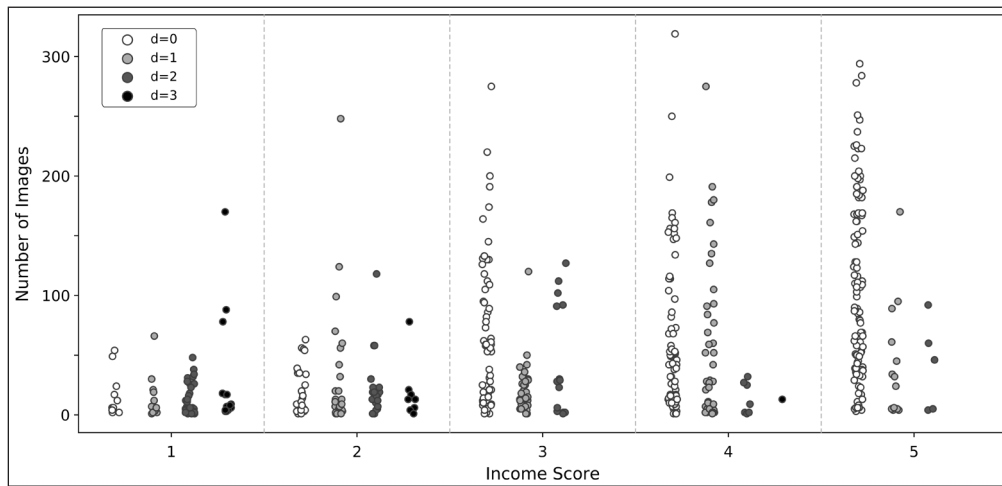
Figure 9 Distribution of predictions by the model indicating the prediction difference of the income score and the number of images per census sector (points). Each income score category includes the 500 census sectors available in Vale do Ribeira. The scale bar shows the difference from 0 (exact match) to 3 (poor match) between the real label and the predicted label (Eq. 3).
